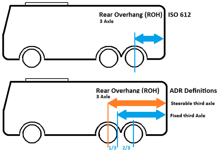
Rear Overhang (ROH) misalignment: International (ISO) vs Australian (ADR)
